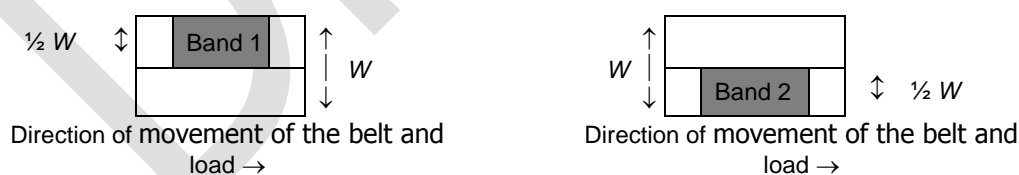
Figure 5.2-1: Positions of load for test of eccentricity.
